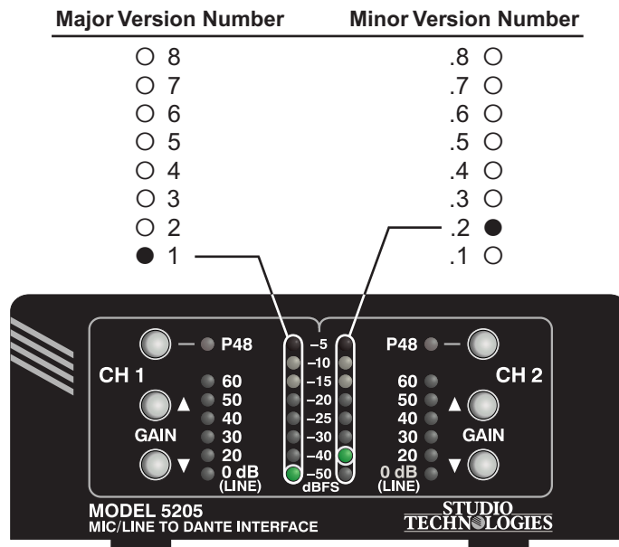
Figure 2. Detail of front panel showing the level meter LEDs that display the application firmware version. In this example, the application firmware version shown is 1.2.
